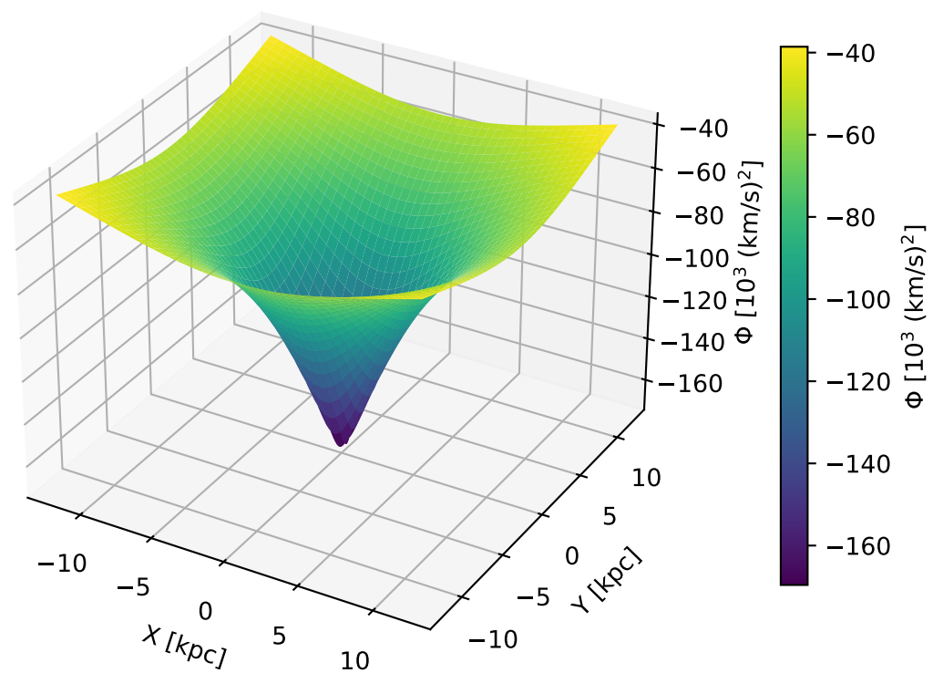
Illustrative Total Potential: MWPotential2014 + Bar + Spiral (z=0.50 kpc)
